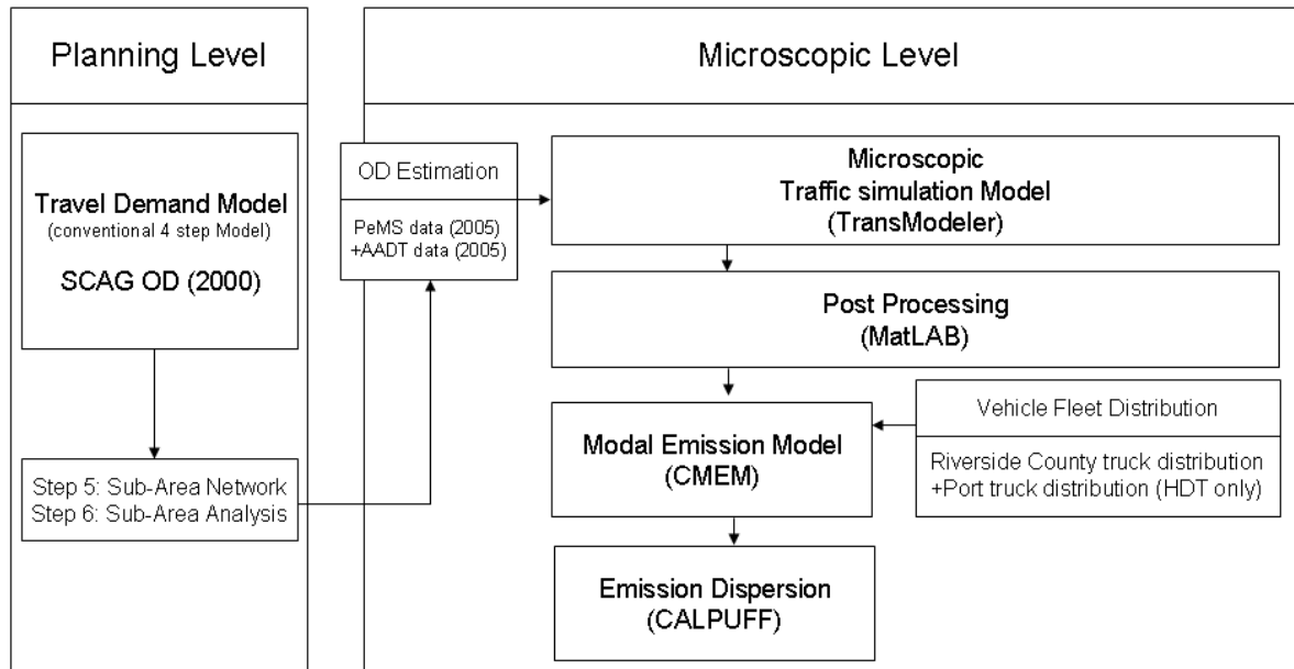
FIGURE 2 Framework for our emissions analyses at the microscopic level.
