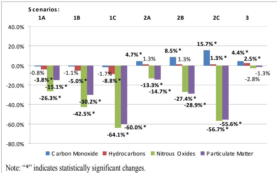
FIGURE 3 Percentage differences in pollutant emissions under each scenario compared to the Base Scenario.
