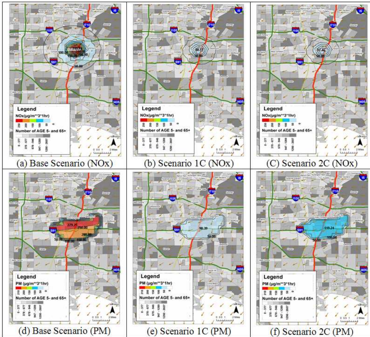
FIGURE 4 NO x and PM dispersion and wind direction for the Base Case, Scenarios 1C and 2C.
