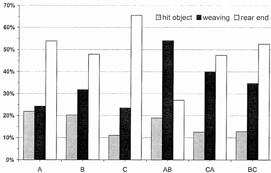
Figure 2 Breakdown of Crash Type for Six Types of Weaving Sections
